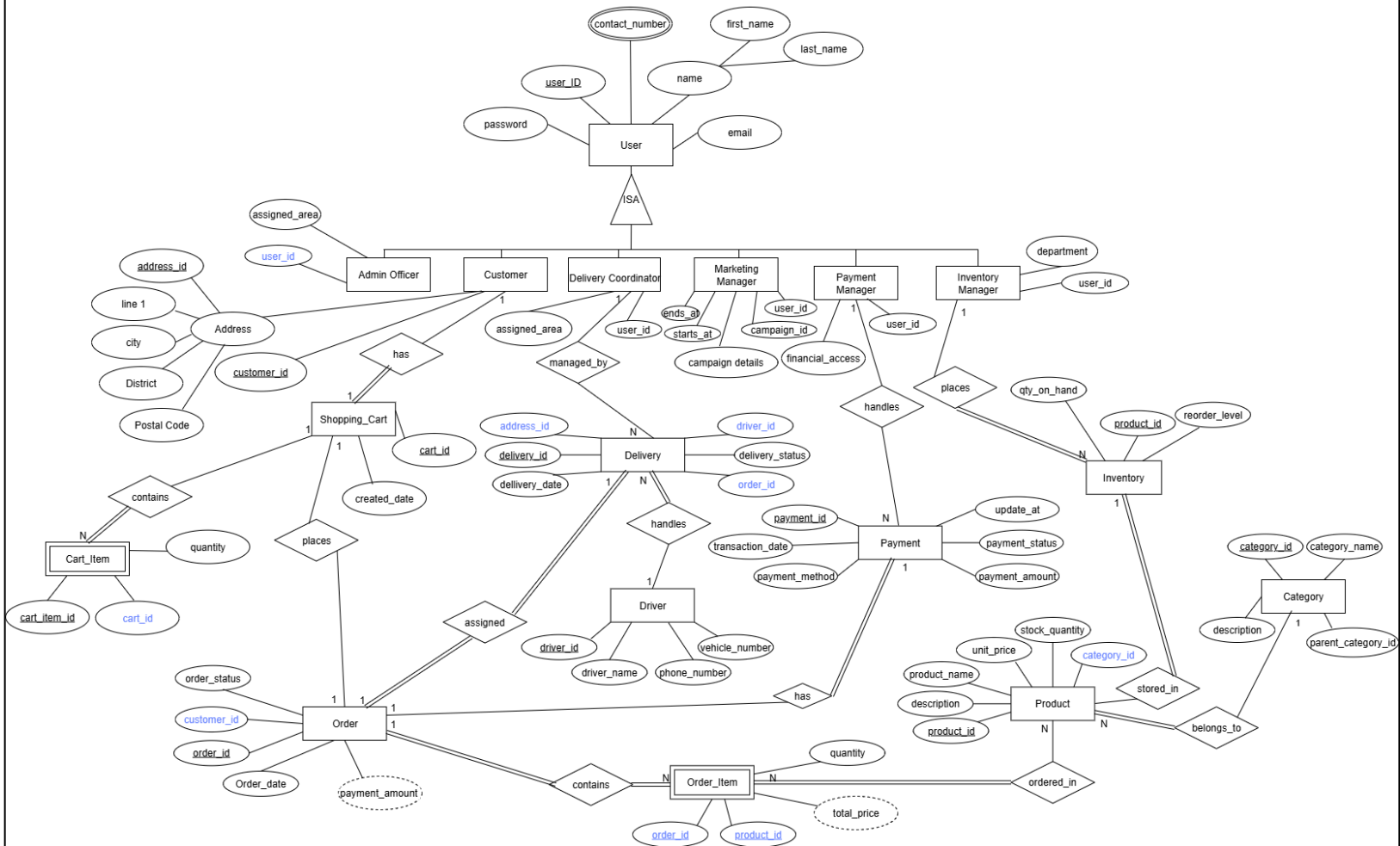
Web-based Supermarket Ordering System
